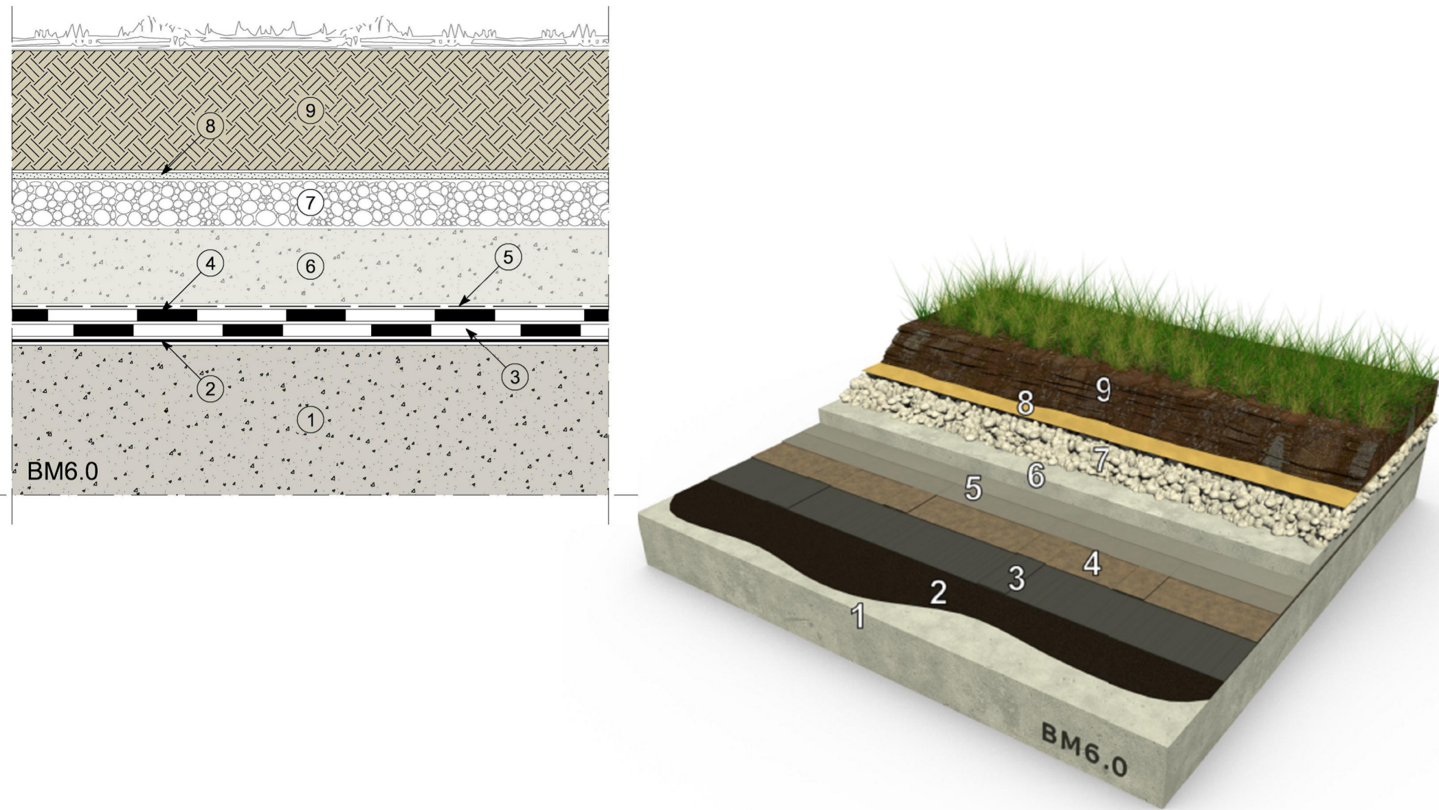
System BM6.0 Green roof with bituminous waterproofing membrane (non-insulated)
